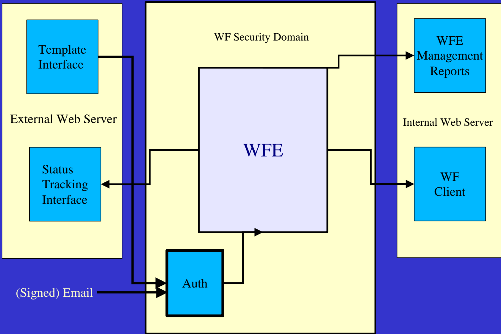
IANA Workflow Management System
